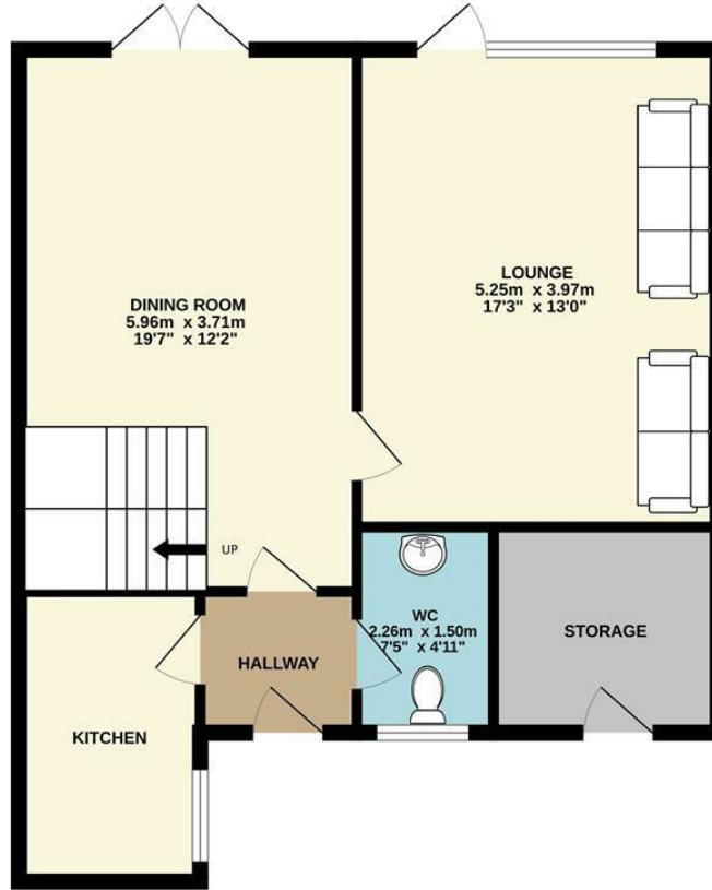
GROUND FLOOR 60.9 sq.m. (656 sq.ft.) approx.
